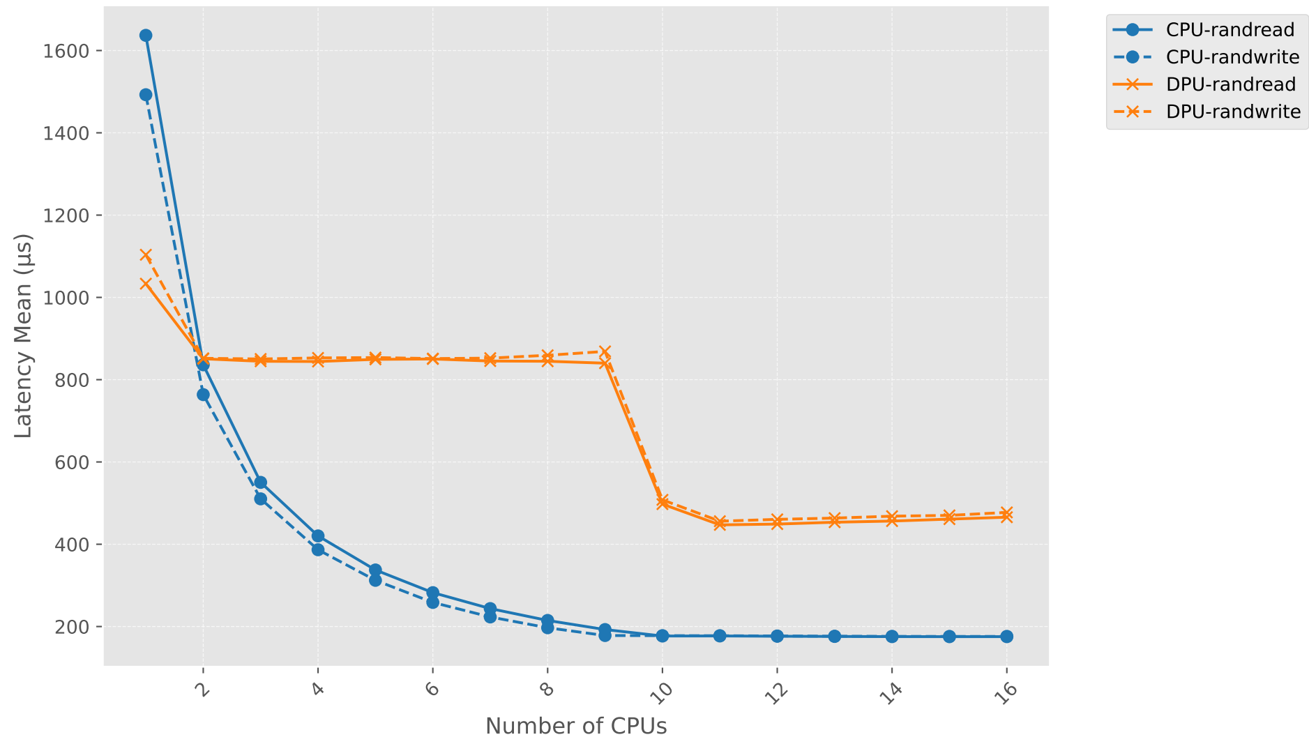
Latency Mean vs Number of CPUs
